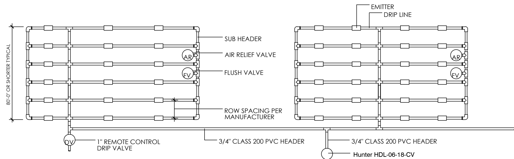
9 TYPICAL DRIP LAYOUT
