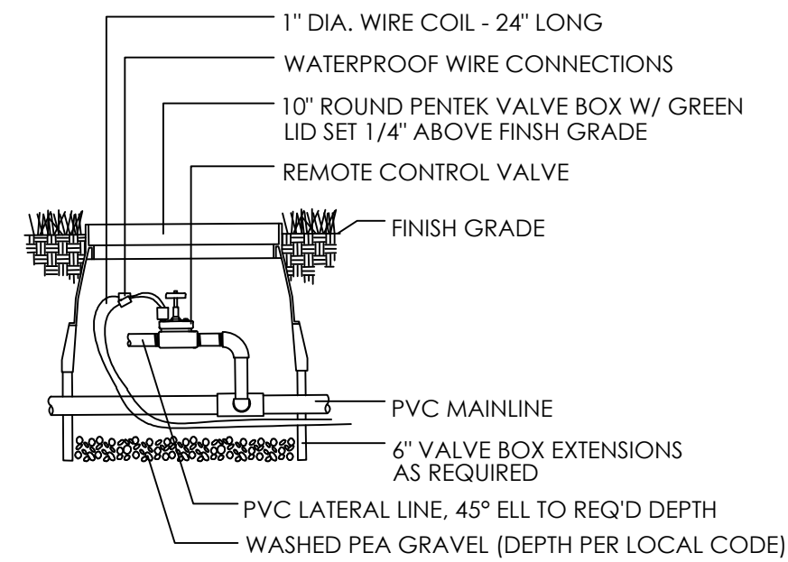
6 REMOTE CONTROL VALVE
