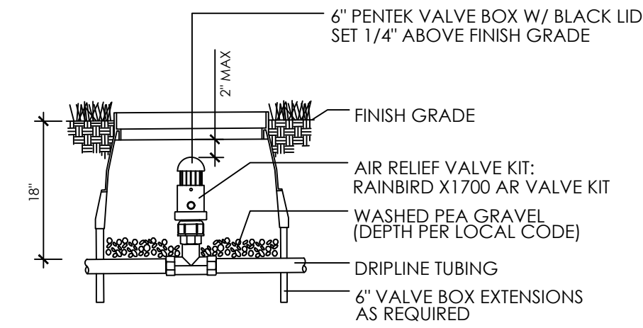
4 AIR RELIEF VALVE
