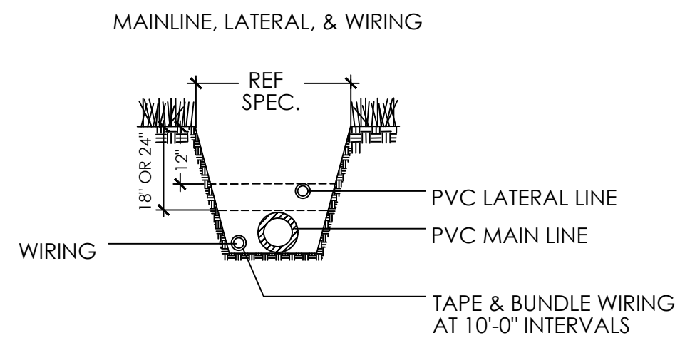
5 TRENCHING DETAIL
