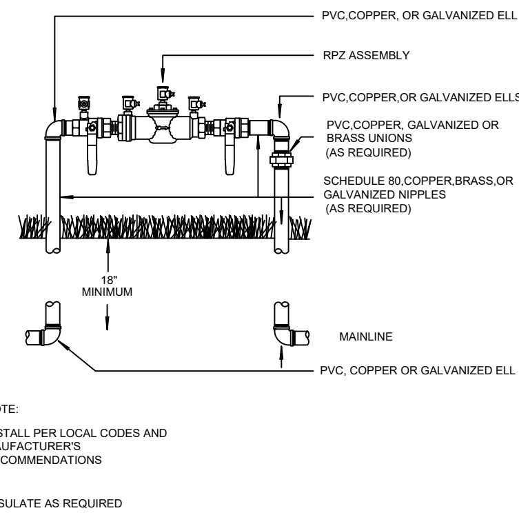
7 RPZ BACKFLOW PREVENTER
