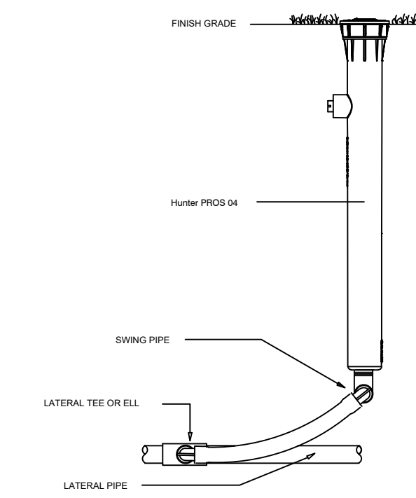
1 POP-UP SPRAY SPRINKLER
