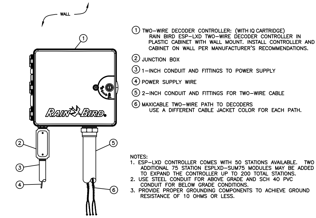
8 ESP-LXD TWO-WIRE DECODER CONTROLLER
